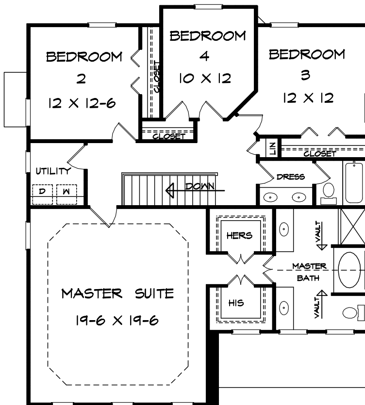
UPPER LEVEL FLOOR PLAN - A
