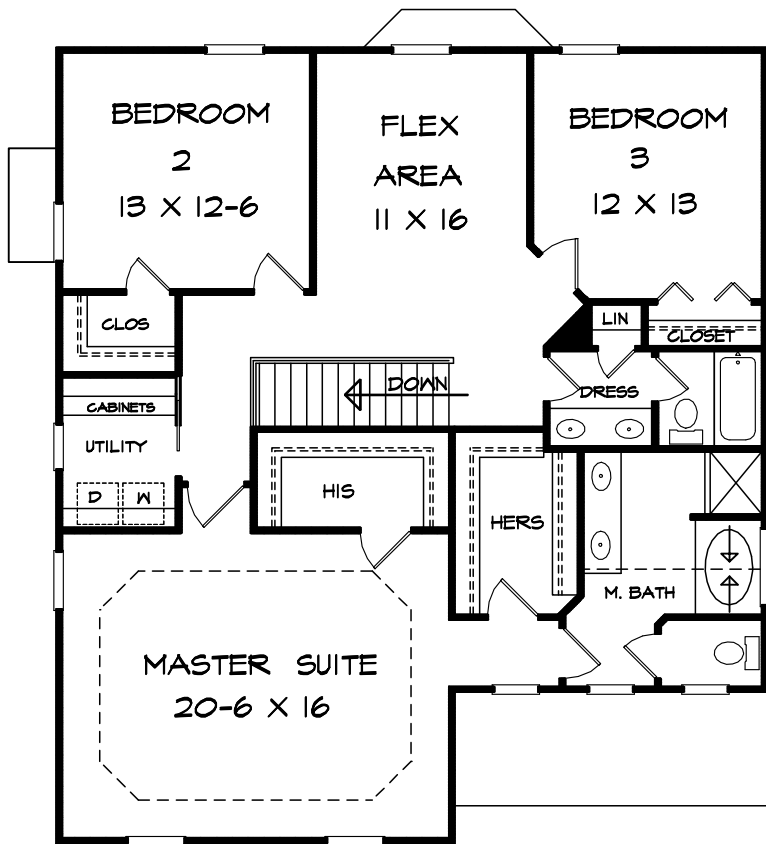
UPPER LEVEL FLOOR PLAN - C
