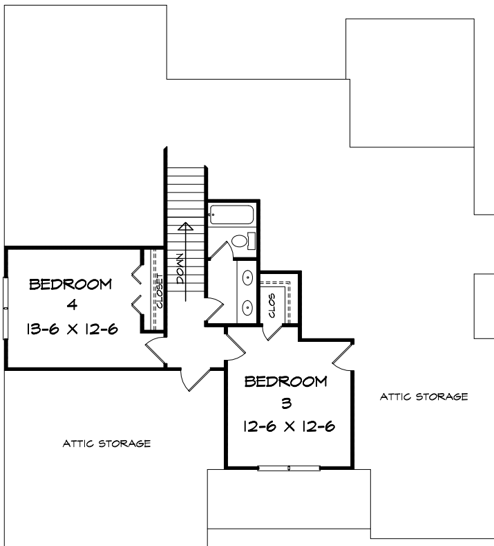
UPPER LEVEL FLOOR PLAN - A
