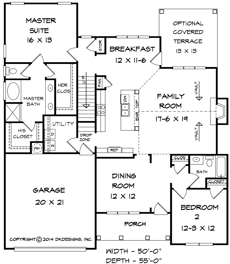
MAIN LEVEL FLOOR PLAN - A
