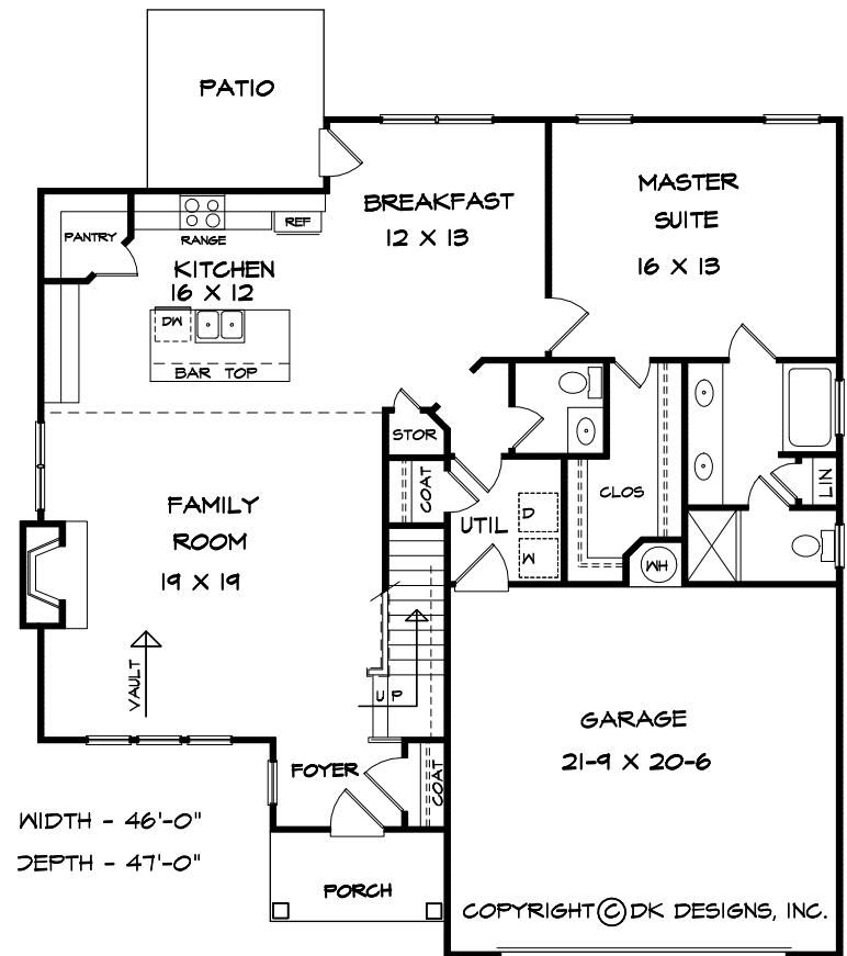
FIRST FLOOR PLAN C
