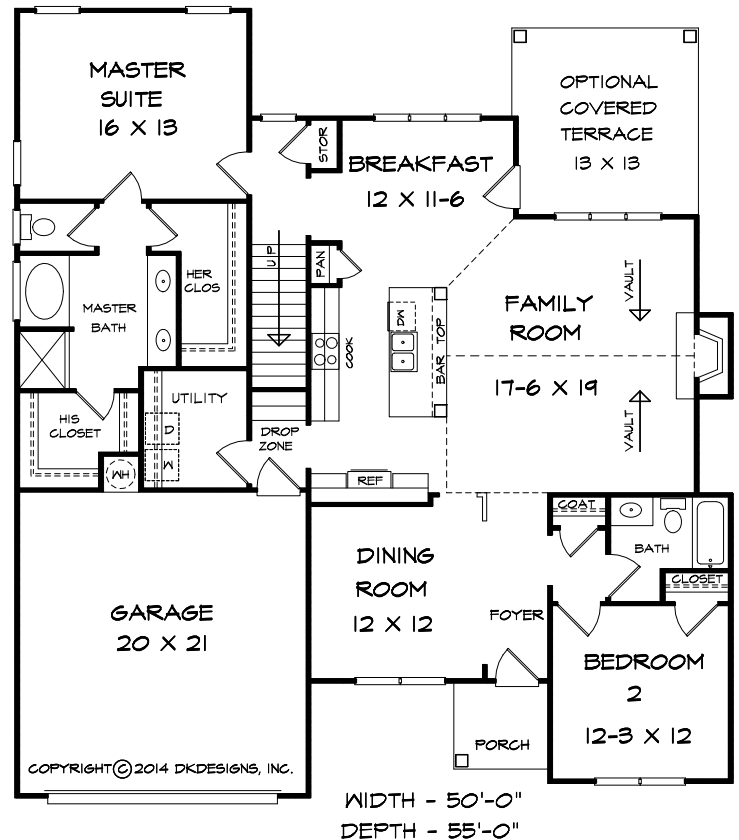
MAIN LEVEL FLOOR PLAN - C
