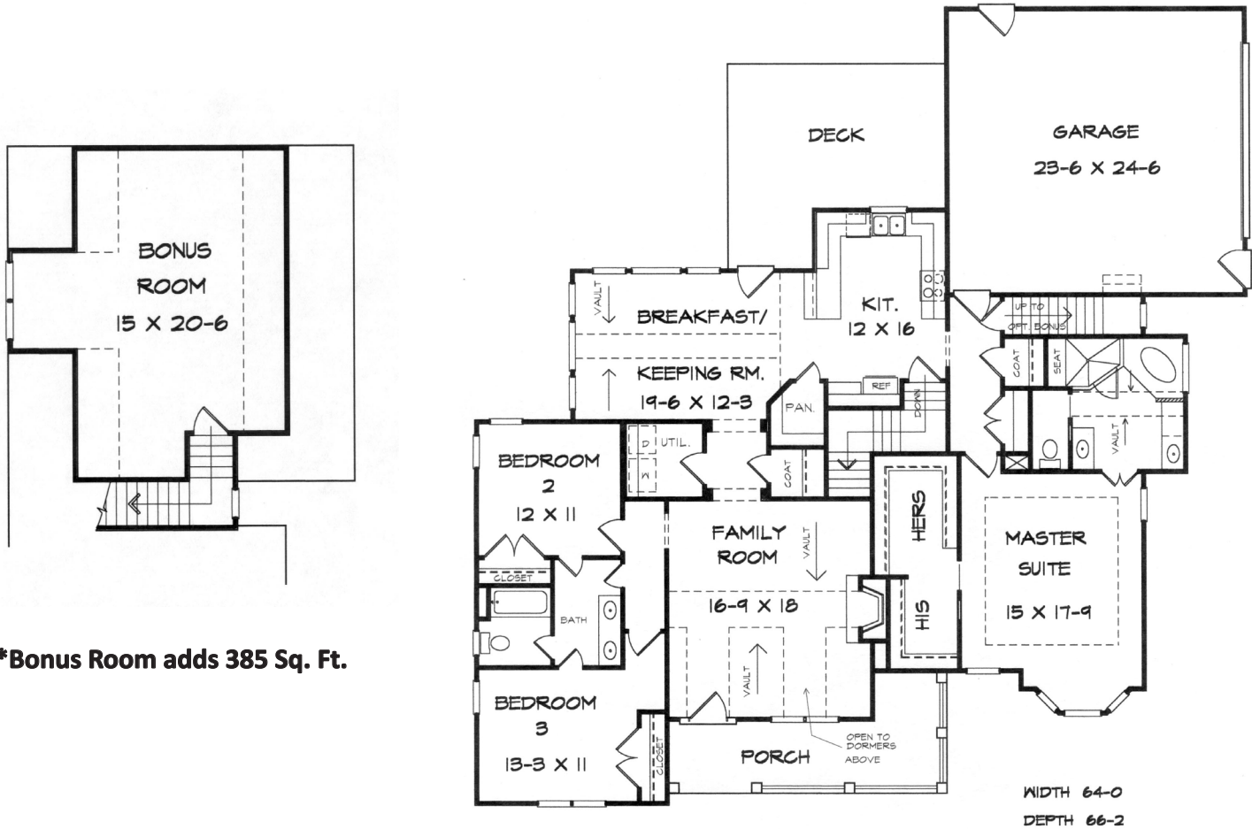
FLOOR PLAN
