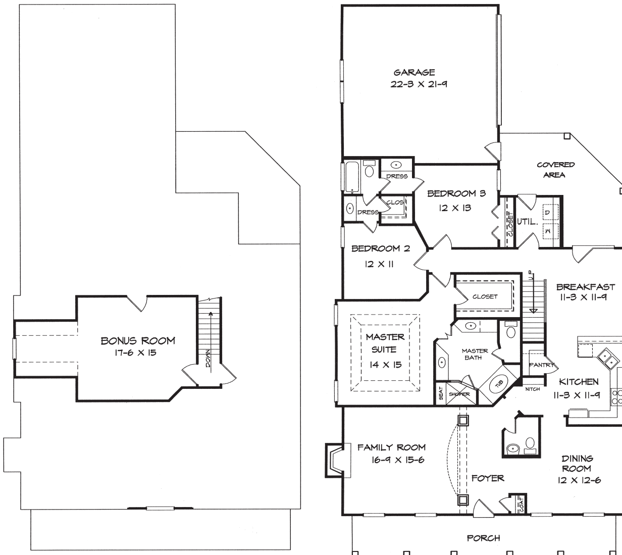
FLOOR PLAN
