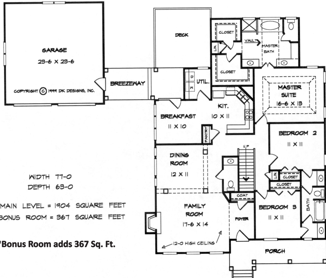
FLOOR PLAN
