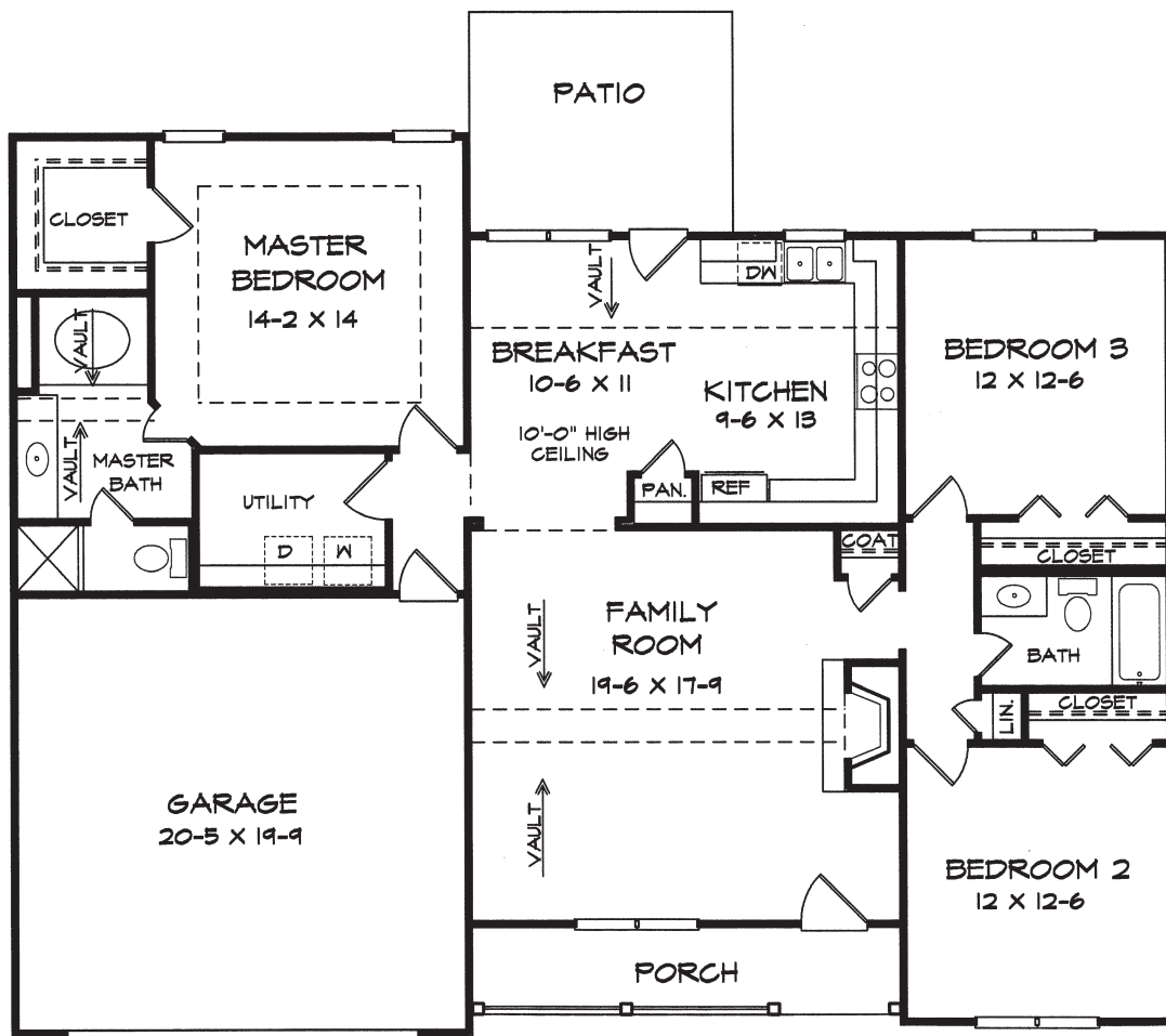
FLOOR PLAN
