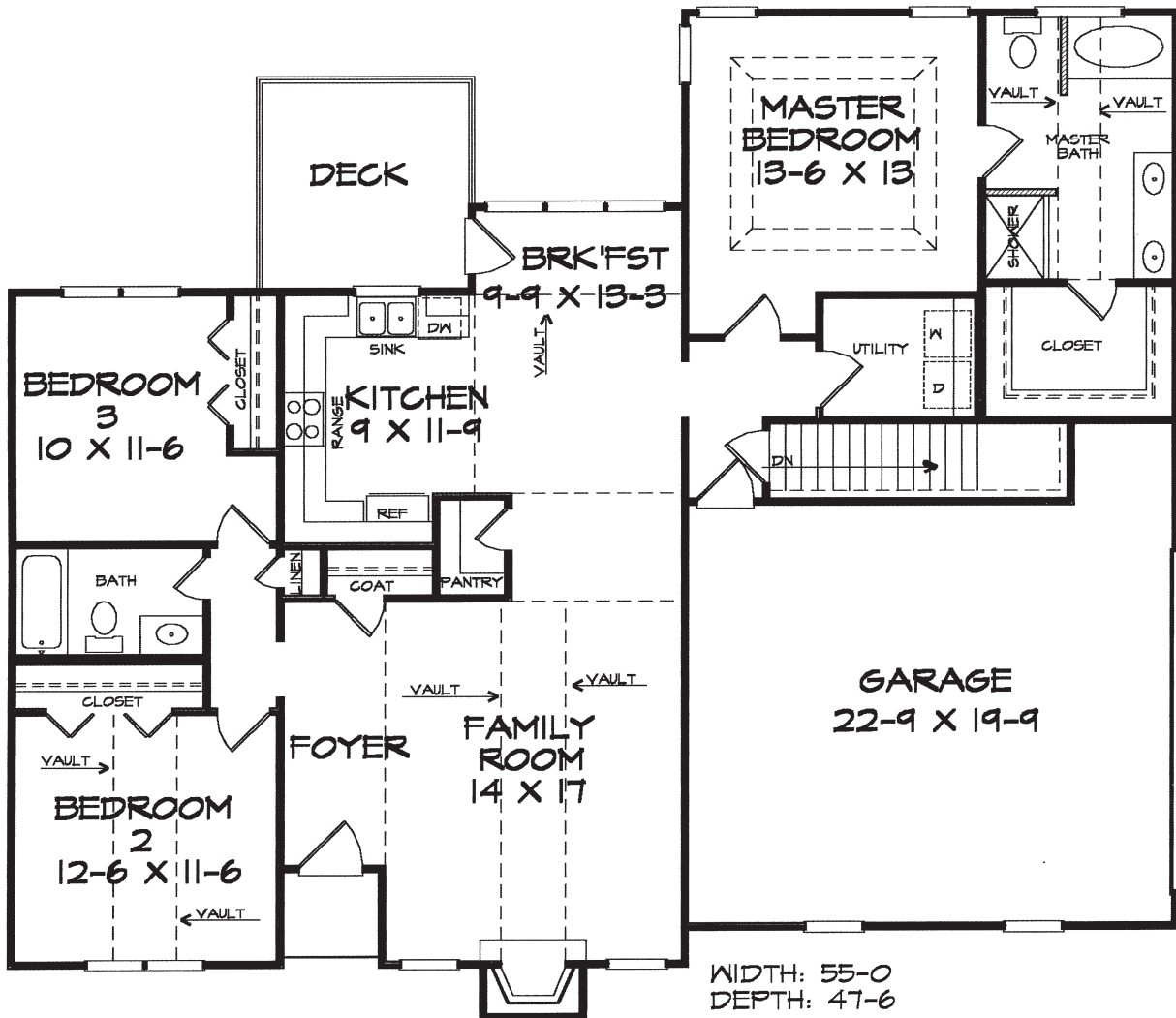
FLOOR PLAN
