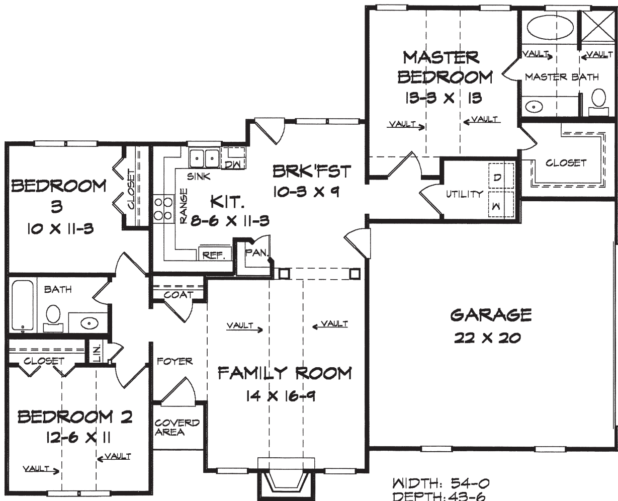
FLOOR PLAN
