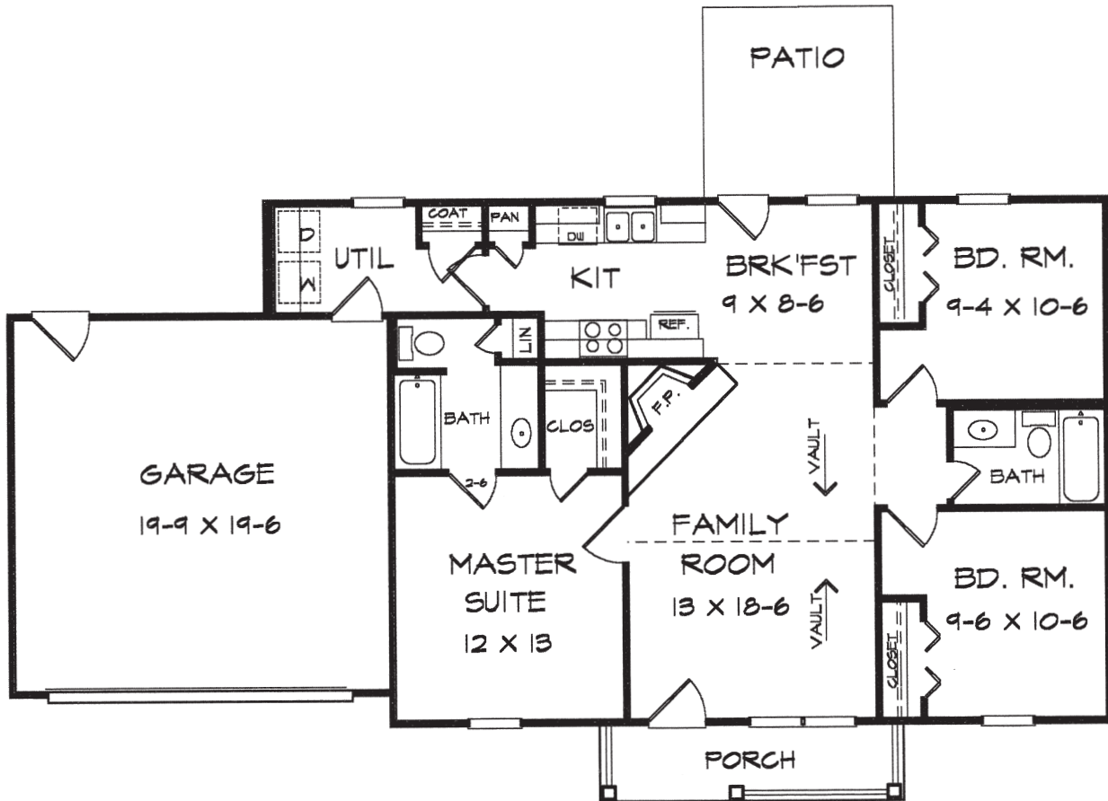
FLOOR PLAN
