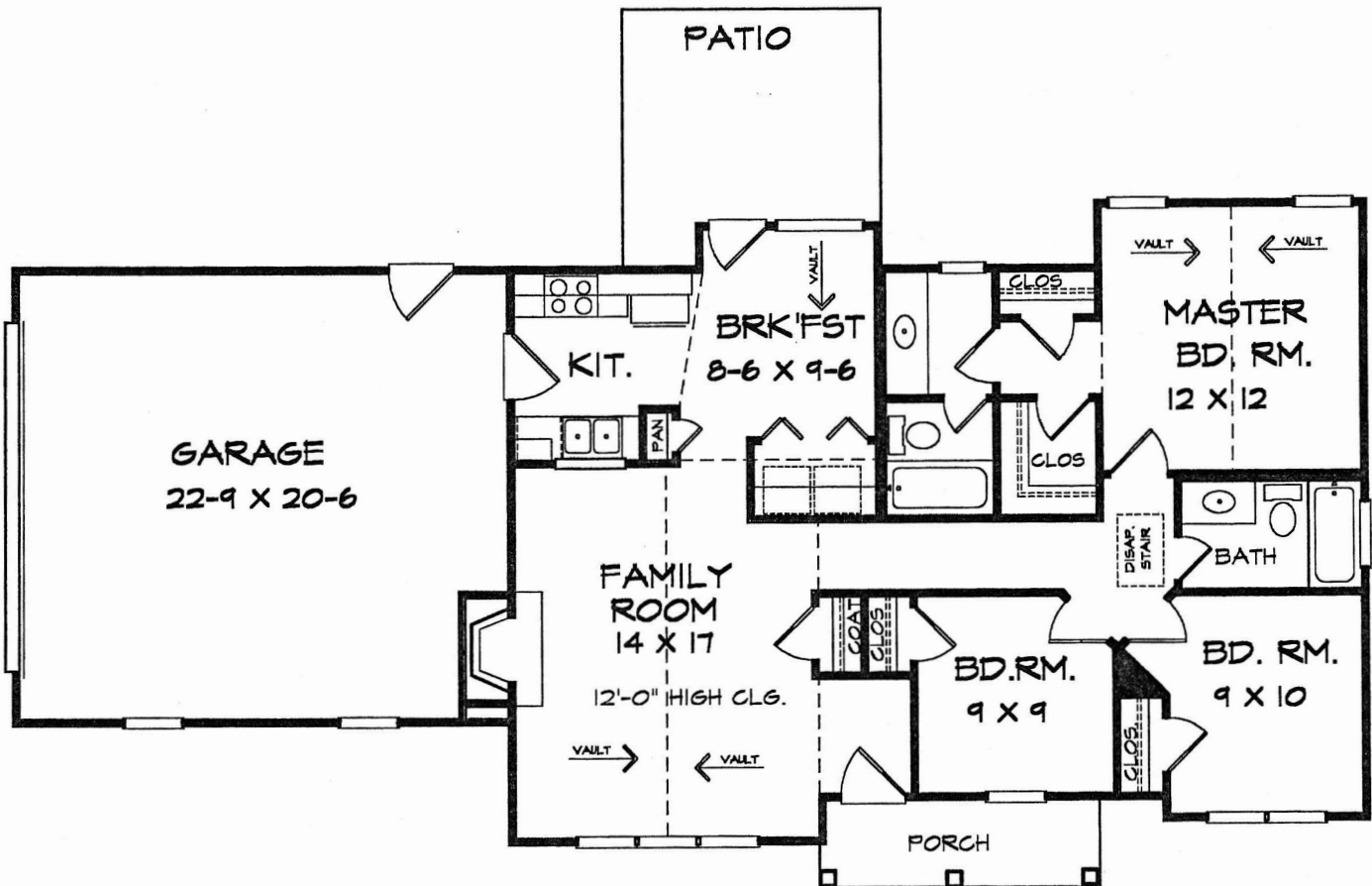
FLOOR PLAN
